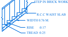
STAIR DETAIL
