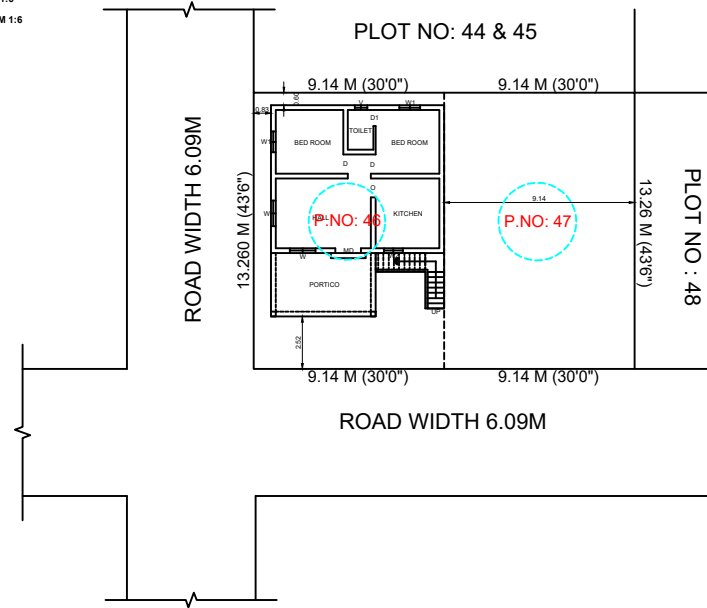
SITE PLAN (SCALE 1:133)
