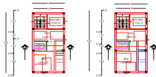
PRO.GROUND FLOOR PLAN
