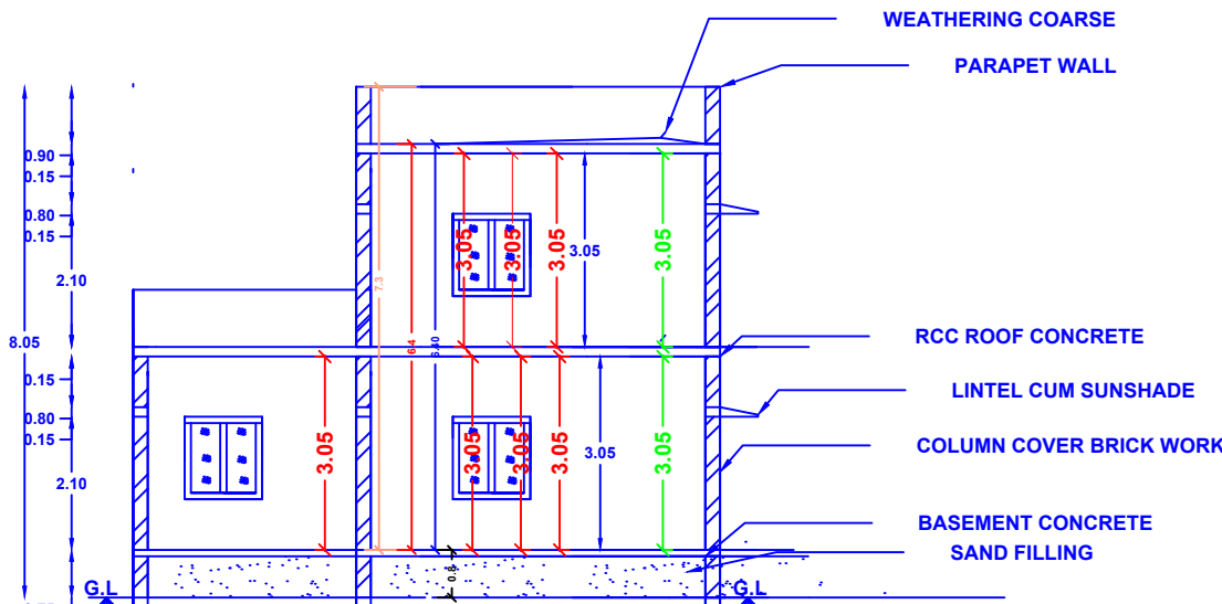
SECTION AB
