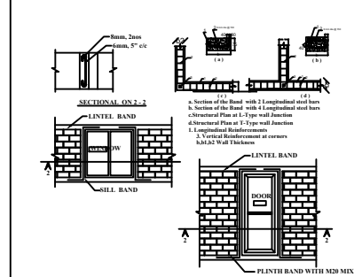
Figure - 2 Reinforcement and Banding Details of Scientific Bands.
