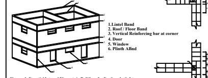
Figure - 1 Essential Elements in Buildings for Earthquake Safety.
