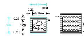
DETAILS OF FILTER BED & WELL
