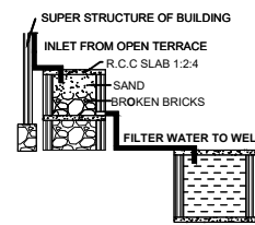
RAINWATER HARVESTING
