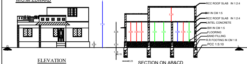
SECTION ON AB&CD
