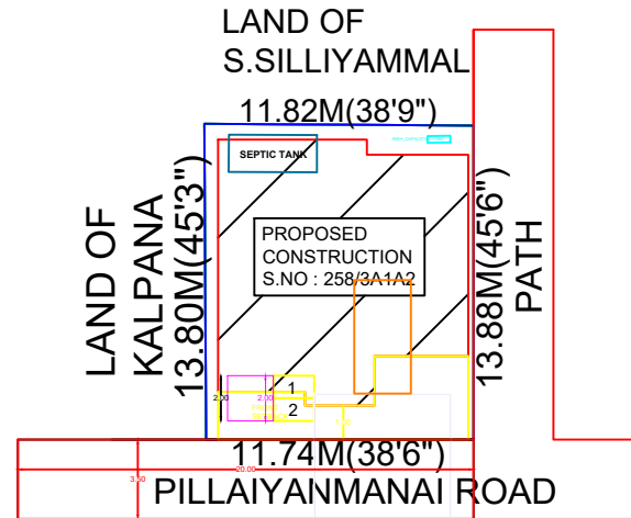
SITE PLAN
