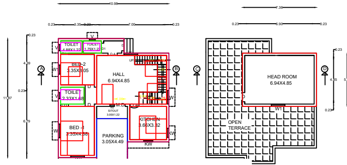
ROOM PLAN
