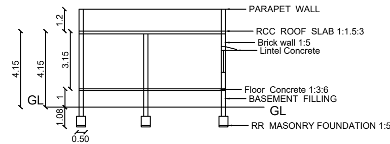
SECTION A-A VIEW
