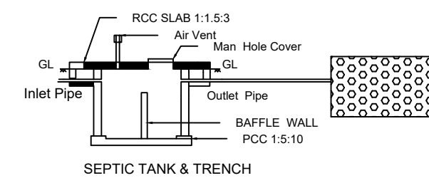
SEPTIC TANK &amp; TRENCH
