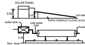
Details of solar water heating system
