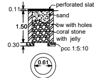
percolation pit
