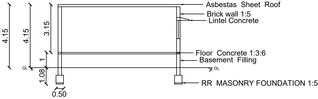
SECTION A-A VIEW
