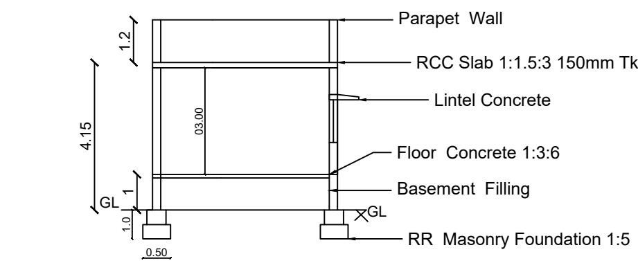
SECTION A - A VIEW
