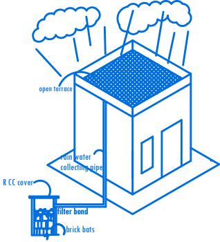
RAIN WATER HARVESTING ARRANGEMENT
