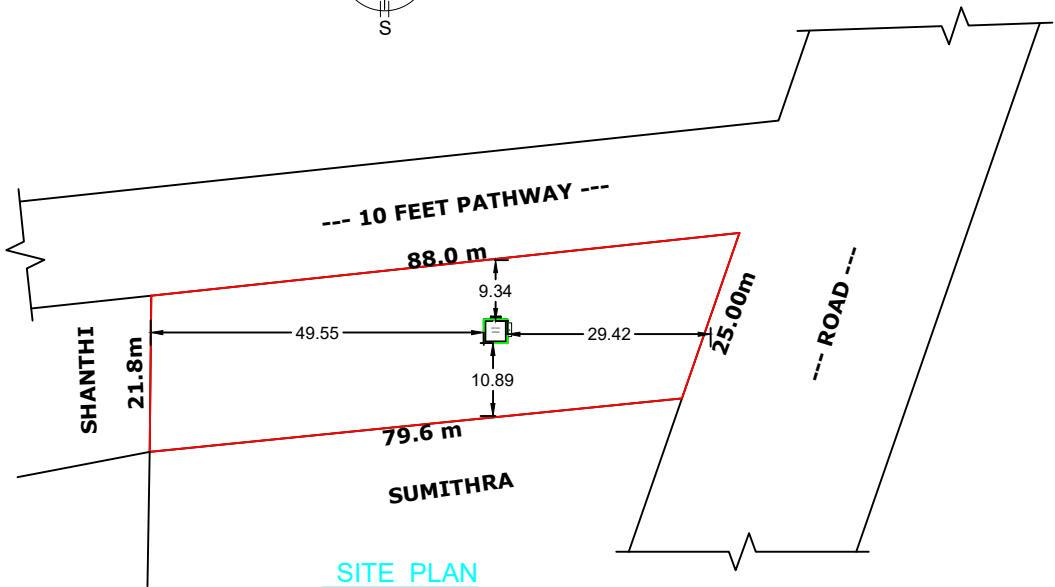
SITE PLAN (SCALE 1:800)
