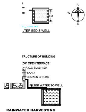
RAINWATER HARVESTING
