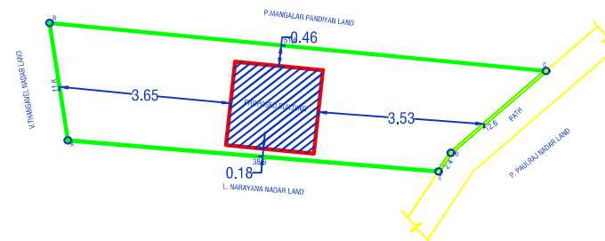
SITE PLAN
