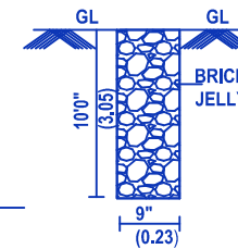
PERCULATION PIT
