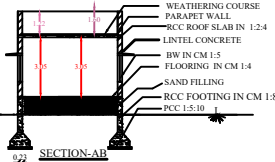
SECTION-A-B
