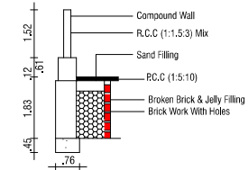
RAIN WATER HARVEST DETAILS
