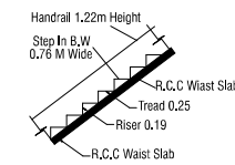
STAIRCASE DETAIL
