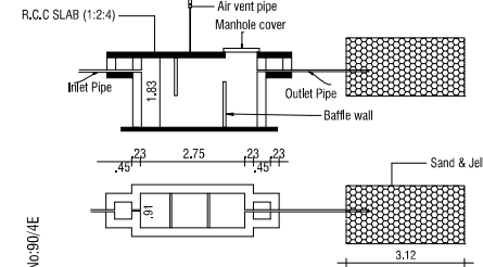
SEPTIC TANK & TRENCH
