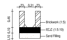
DETAILS OF DRAINAGE PIT
