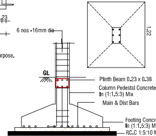
COLUMN & FOOTING DETAILS
