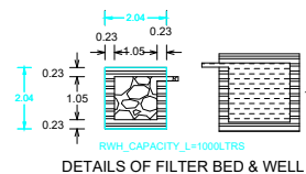
DETAILS OF FILTER BED & WELL
