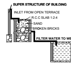
RAINWATER HARVESTING
