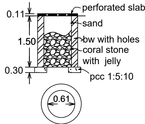
PERCOLATION PIT
