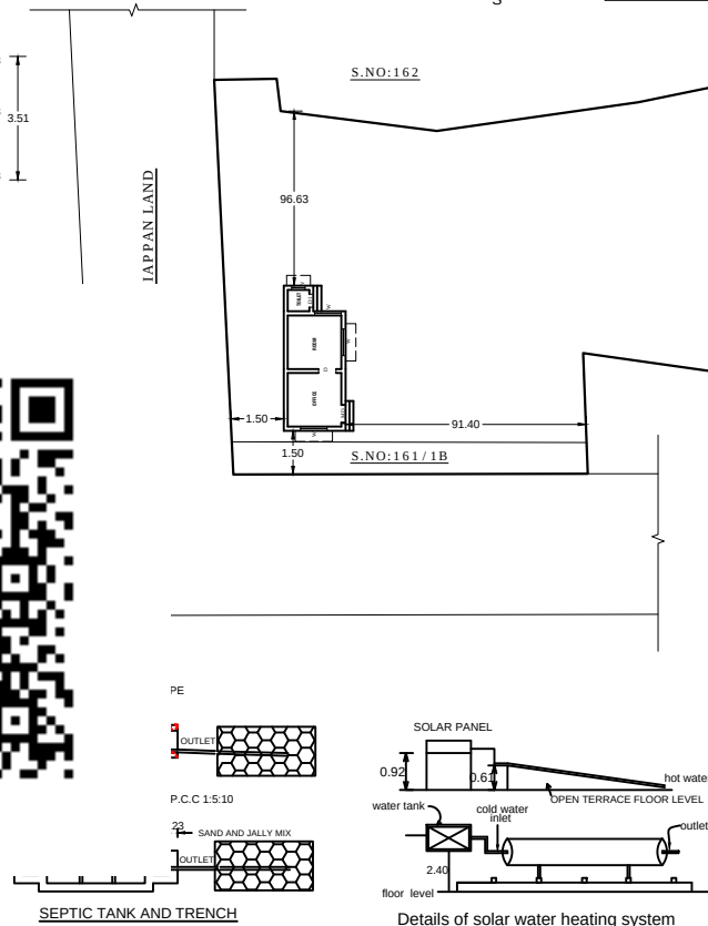
Details of solar water heating system
