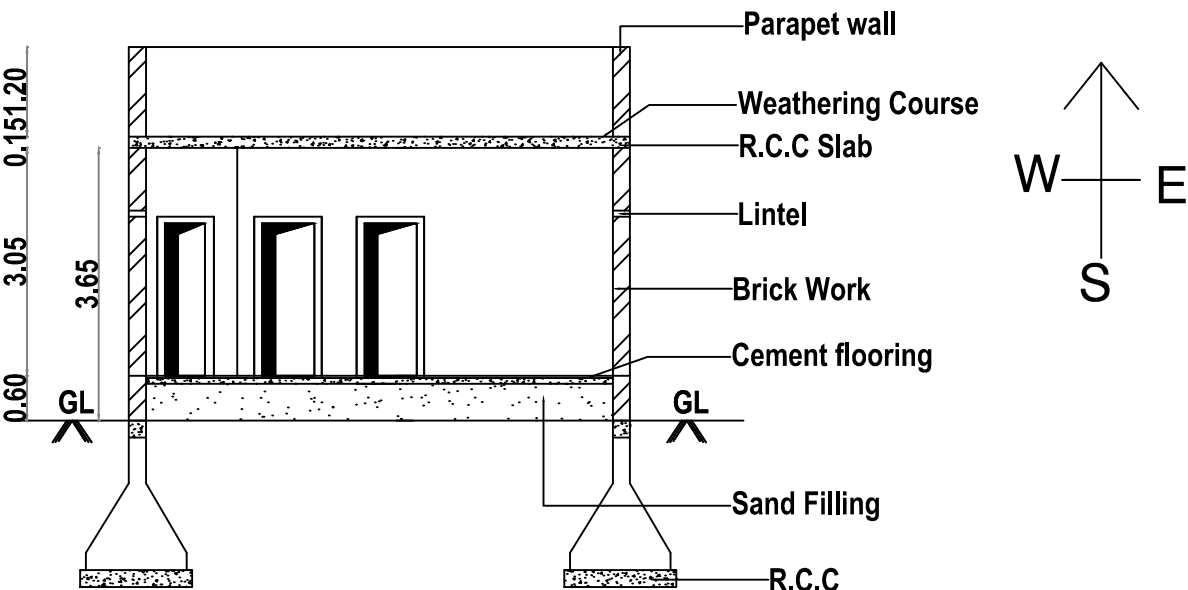
CROSS SECTION"AA"
