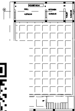
FLOOR PLAN
