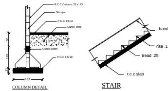
COLUMN DETAIL
