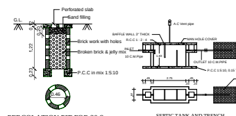
PERCOLATION PIT FOR 30 Sq. m. (Scale:- 1:50)
