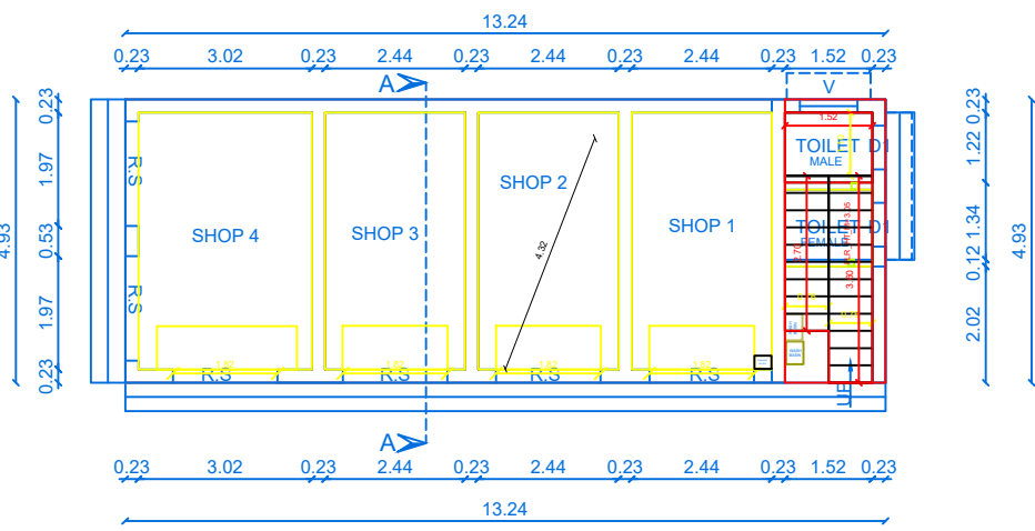
GROUND FLOOR COMMERCIAL SHOP PLAN
