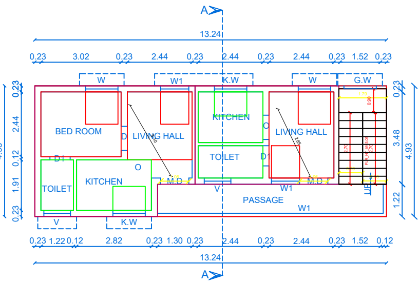
FIRST FLOOR RESIDENTIAL HOUSE PLAN
