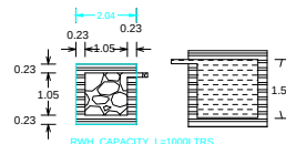
DETAILS OF FILTER BED & WELL
