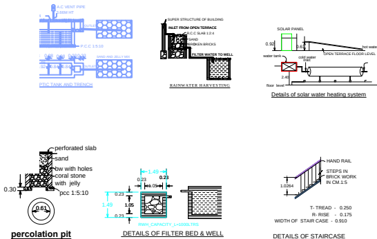
percolation pit
