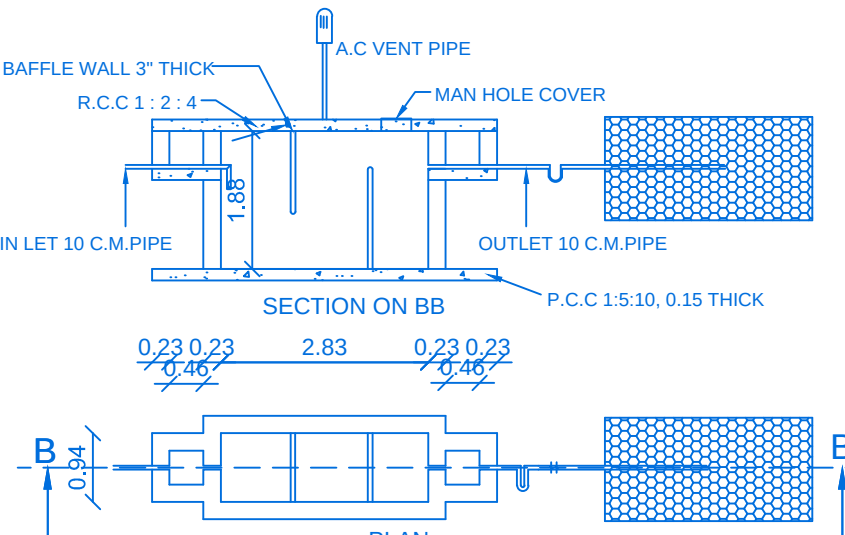
SEPTIC TANK AND TRENCH & U TRAP ADOPTED
