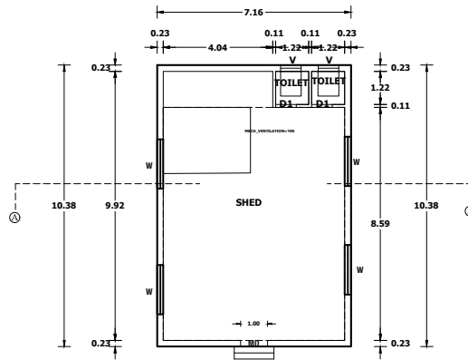
PRO.BLOCK-2 GROUND FLOOR AREA
