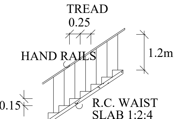
STAIRCASE DETAIL
