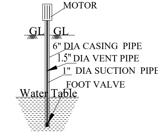
SEC. OF BOREWELL
