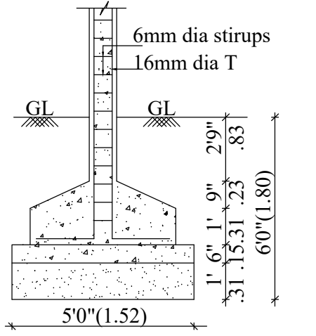
COLUMN FOUNDATION DETAIL SCALE (NTS)
