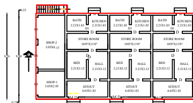
EXG.GROUND FLOOR PLAN
