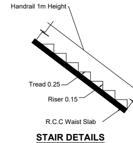
STAIR DETAILS
