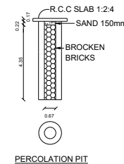
PERCOLATION PIT
