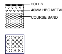
RAIN WATER COLLECTING TANK
