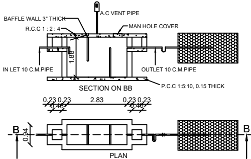
SEPTIC TANK AND TRENCH & U TRAP ADOPTED
