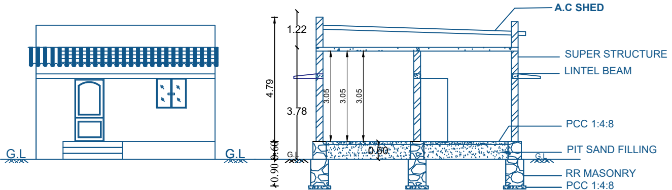
FRONT ELEVATION
