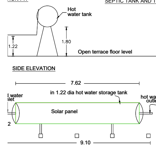
SOLAR WATER HEATER PLANT
