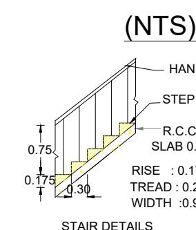
STAIR DETAILS
