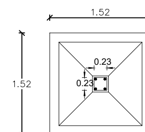
RCC COLUMN DETAILS
