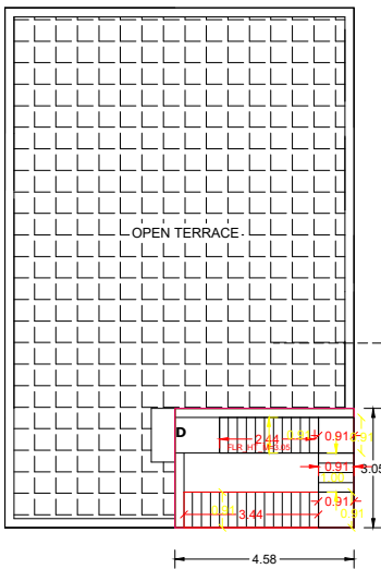
PRO.FIRST FLOOR PLAN
