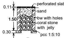
percolation pit
