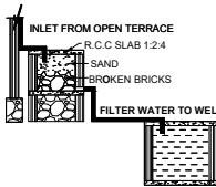
RAINWATER HARVESTING
