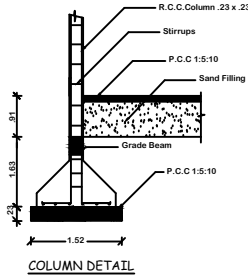
COLUMN DETAIL
