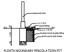
PLINTH BOUNDARY PERCOLATION PIT
