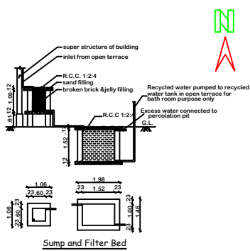
Sump and Filter Bed
