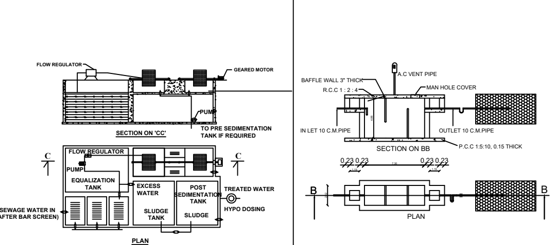
SEPTIC TANK AND TRENCH & U TRAP ADOPTED
