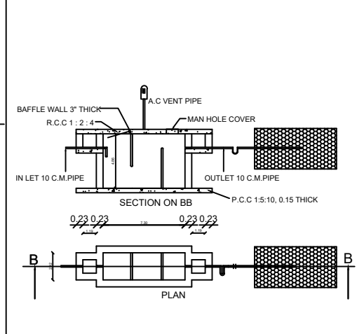
SEPTIC TANK AND TRENCH & U TRAP ADOPTED
