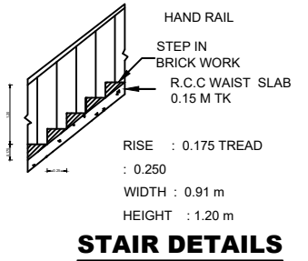
STAIR DETAILS
