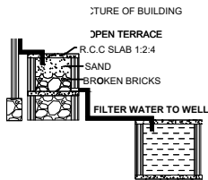
RAINWATER HARVESTING
