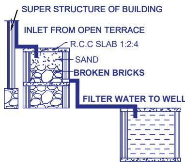
RAINWATER HARVESTING
