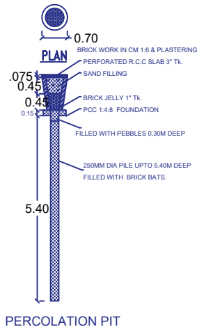
PERCOLATION PIT
