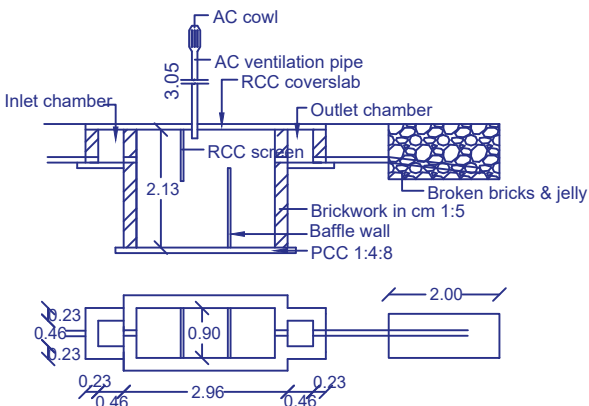
SEPTICTANK DETAILS
