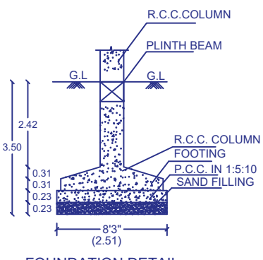
FOUNDATION DETAIL (DETAIL - B)
