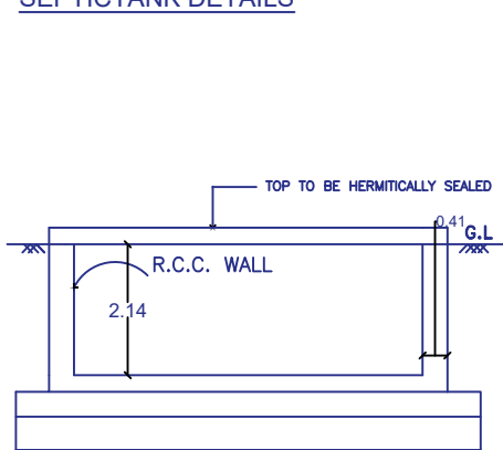
RWH SECTION (SAMPLE) RWH_CAPACITY_L=2000LTRS
