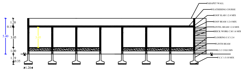
SECTIONAL ELEVATION
