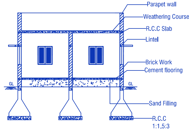
CROSS SECTION ON 'AB'
