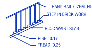
STAIR CASE DETAIL
