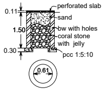
percolation pit
