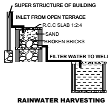
RAINWATER HARVESTING
