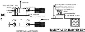
RAINWATER HARVESTING
