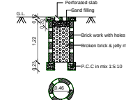
PERCOLATION PIT FOR 30 Sq. m. (Scale:- 1:50)
