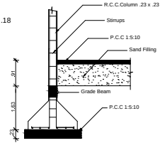
COLUMN DETAIL
