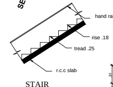
STAIR
