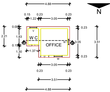
PROPOSED PLAN
