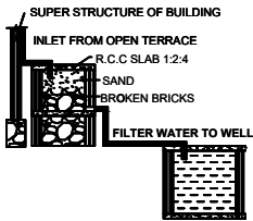
RAINWATER HARVESTING
