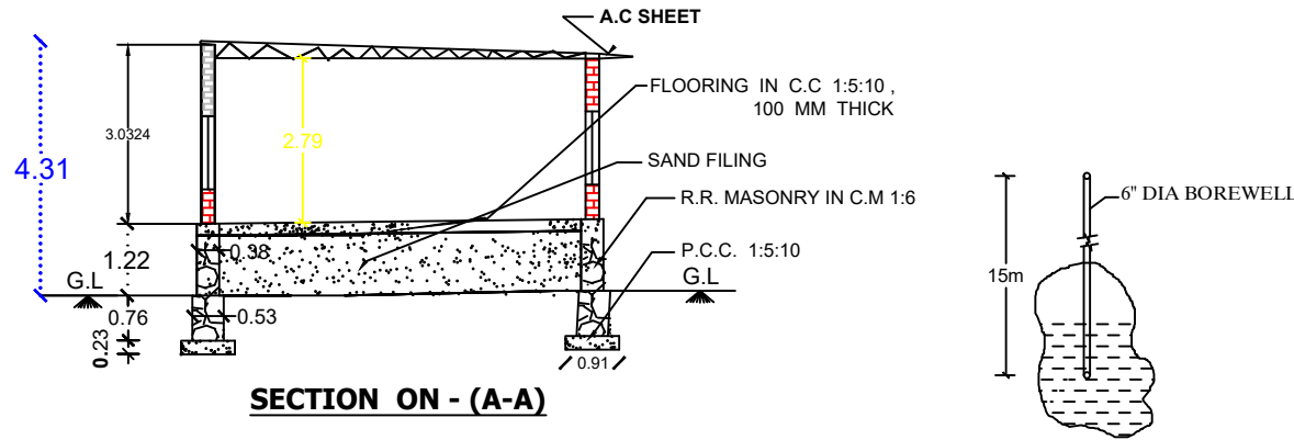
BORE WELL DETAIL
