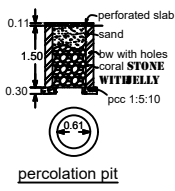
percolation pit
