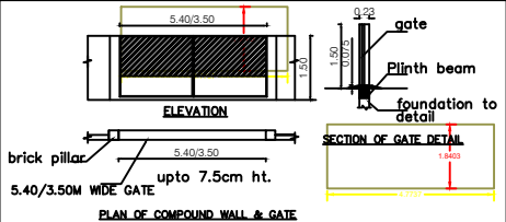
PLAN OF COMPOUND WALL & GATE
