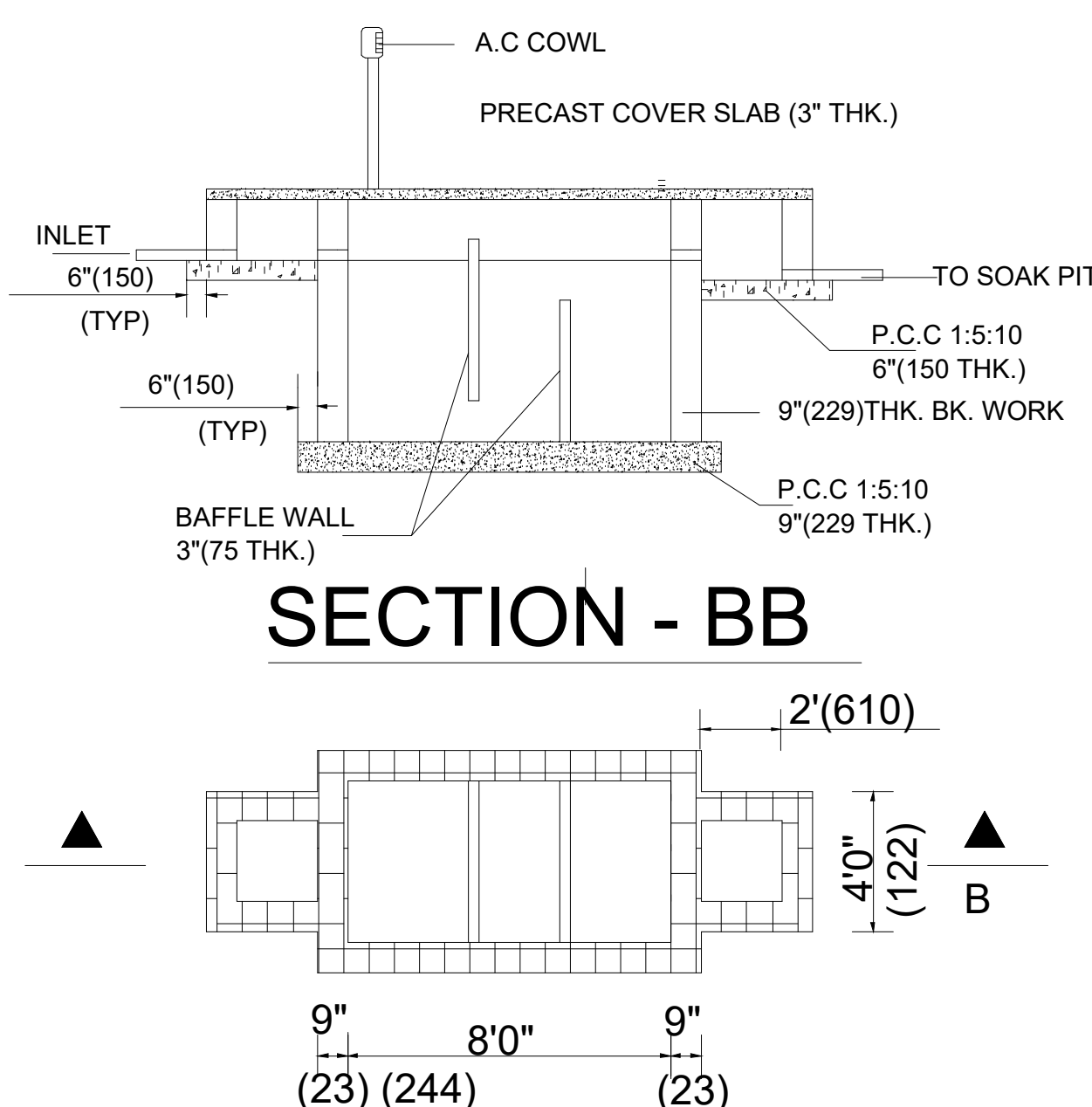
PLAN OF SEPTIC TANK
