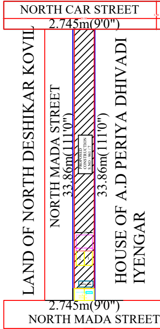
EXG & PRO-F.FLOOR PLAN
